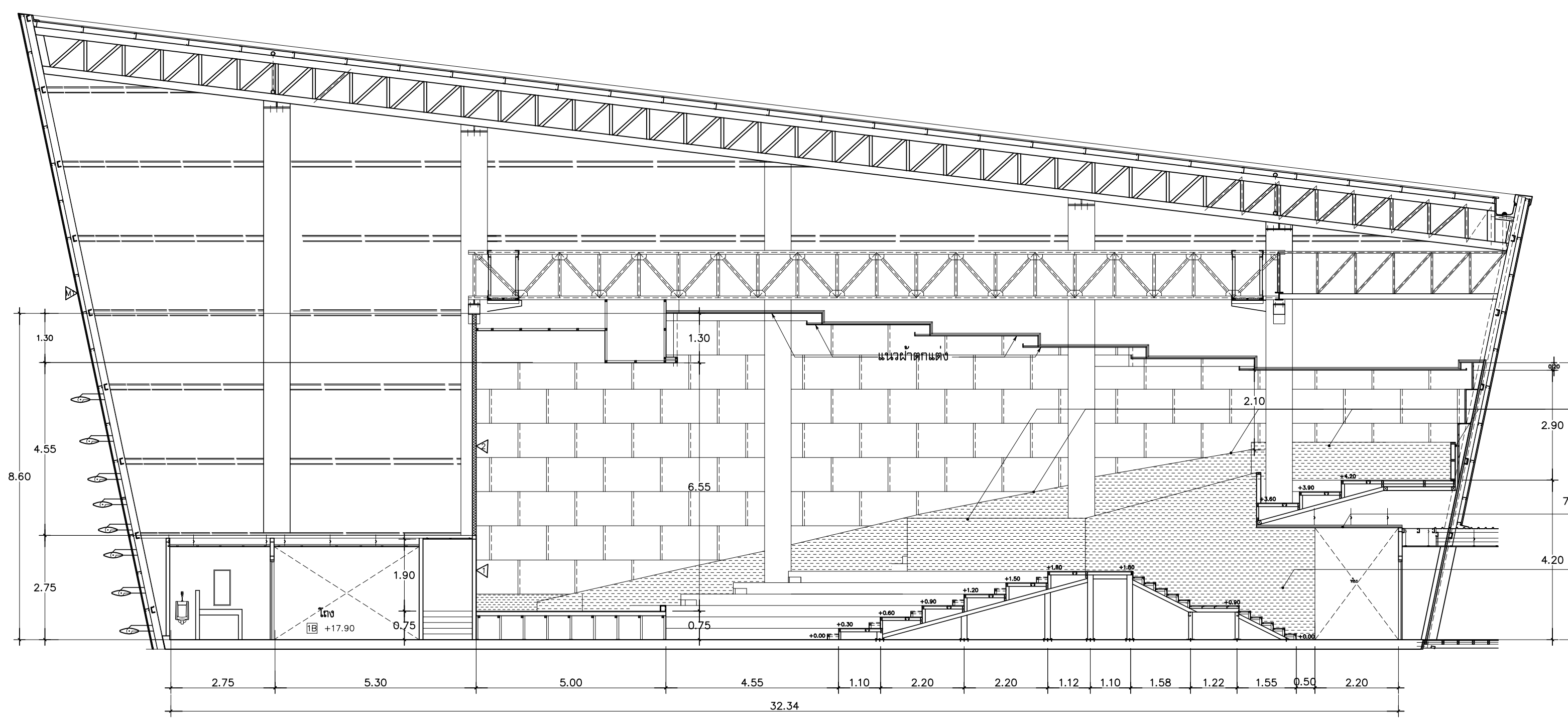
SECTION 2 SCALE 1:100 A5-01
